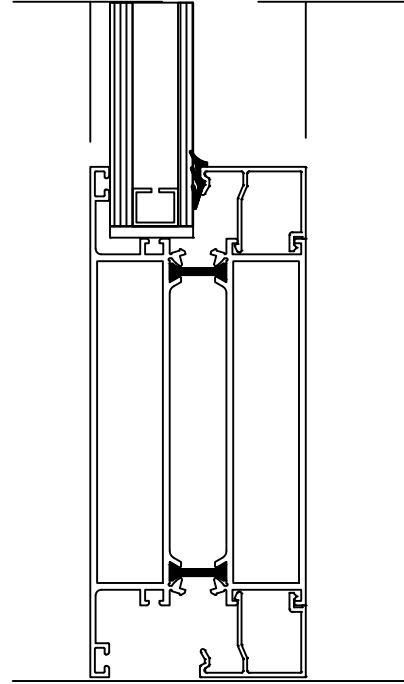
DETAY 5 SABİT ETEK DETAYI
