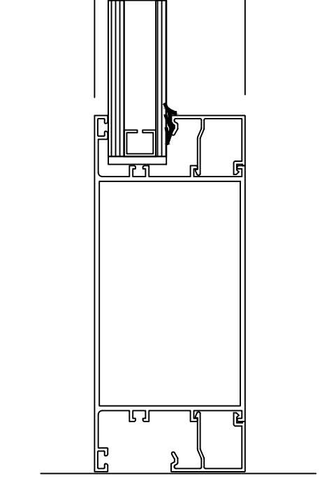
DETAY 5 SABİT ETEK DETAYI
