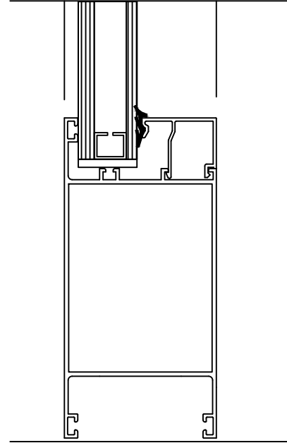
DETAY 23 SABİT ETEK DETAYI
