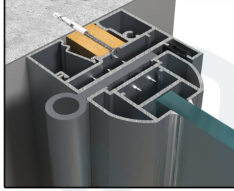
D47_KAPI KASA + OVAL CAM KANAT DETAYI
