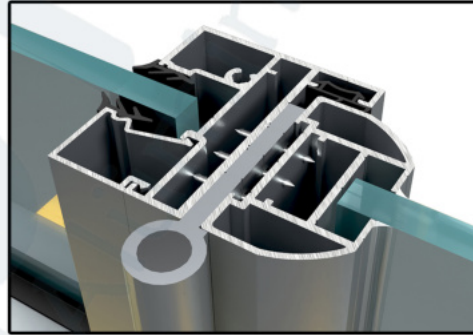
D49_SABİT CAMLI KAPI KASA + OVAL CAM KANAT DETAYI
