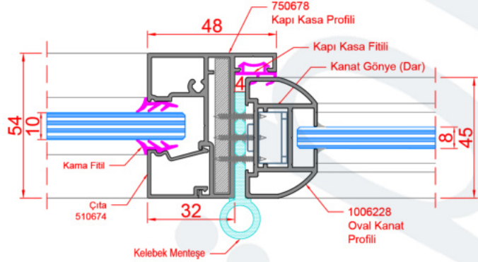
D49_SABİT CAMLI KAPI KASA + OVAL CAM KANAT DETAYI
