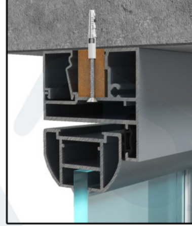
D51_TAVAN KAPI KASA + OVAL CAM KANAT DETAYI
