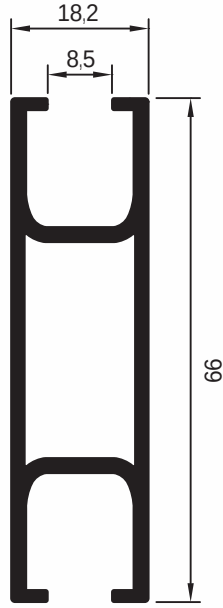
pr no:680629/59 0.910 gr/m
