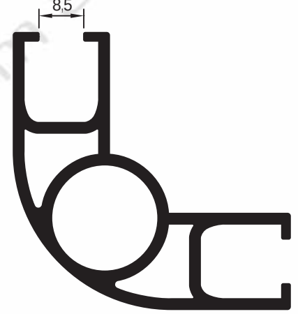
pr no:680628/59 1.280 gr/m
