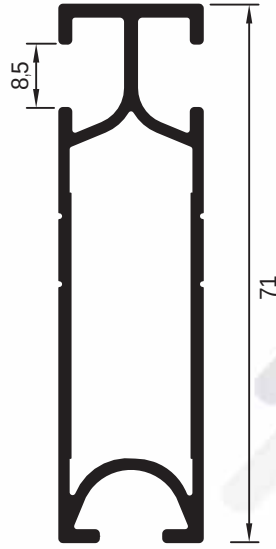
pr no:580690/59 0.790 gr/m
