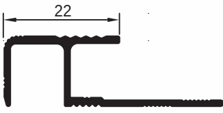
pr no:560662/109 0.250 kg/m
