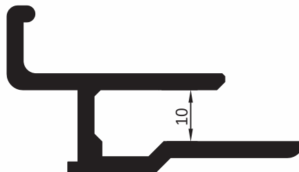
pr no:510672/10 0.894 gr/m
