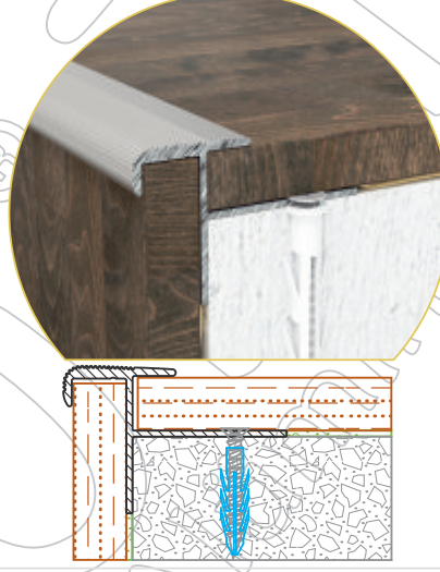
520690 - Basamak profilleri
